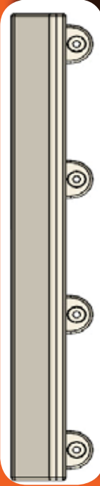
RediKerb SP Straight 150mm wide x 1000mm long 125mm High 10.5kg Weight 4 Fixings
